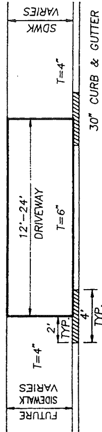
DRIVEWAY DETAIL NO BOULEVARD
